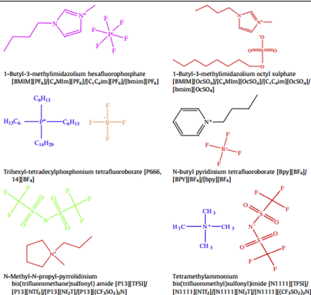
Figure 1. Examples of some common ionic liquids with their formula structures and abbreviations.
